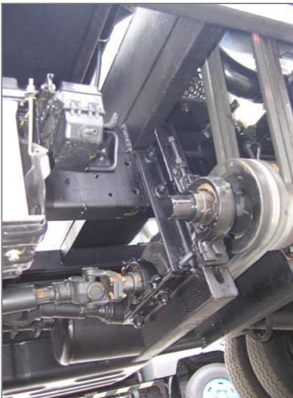
PTO Pulley-Belt drive to protect the pump
